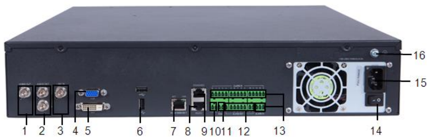
NVR308-32-IN
